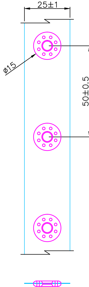
Female Part Art.nr. PT0011F
