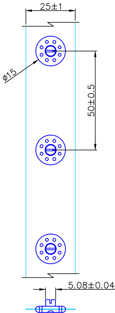
Male Part Art.nr. PT0011M
